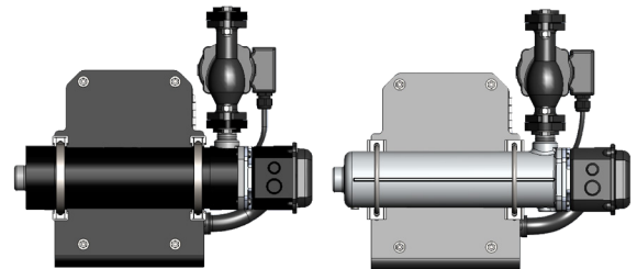
Figure 2 (Above). Rear-view of Hotstart CSM (type B) heating system showing tank assembly with sleeve (left) and without sleeve (right).
